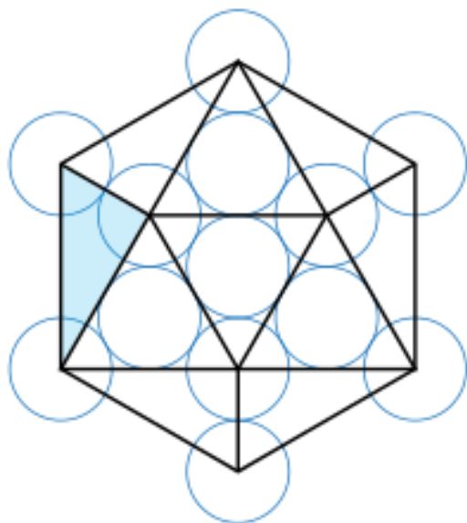
Icosahedron
