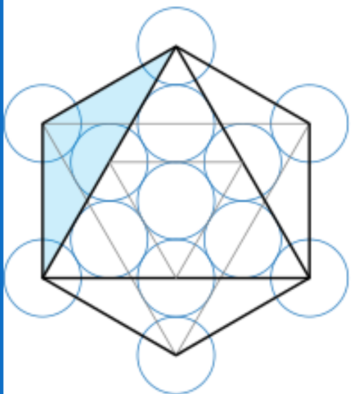
Octahedron
