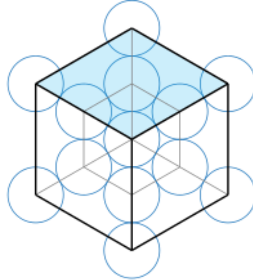
Hexahedron (Cube)
