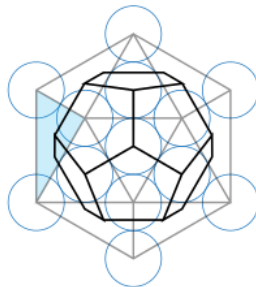
Dodecahedron
