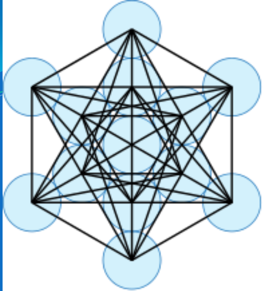
Metatron's Cube
