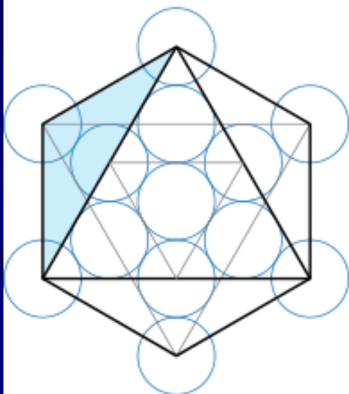
Octahedron
