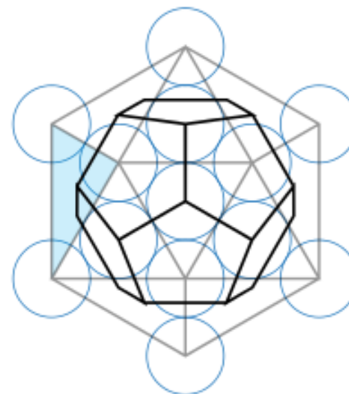
Dodecahedron
