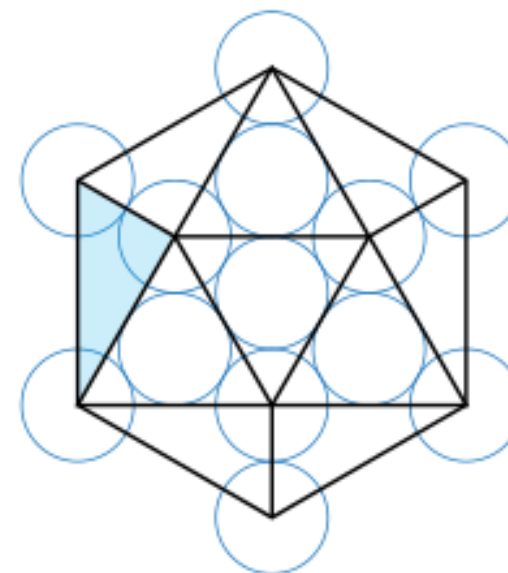
Icosahedron
