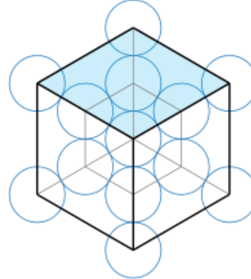
Hexahedron (Cube)
