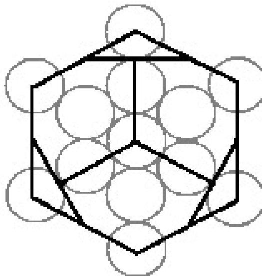
Dodecahedron
