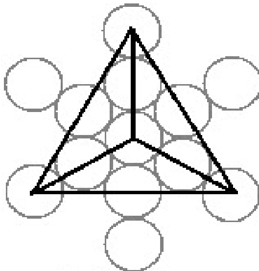
Tetrahedron
