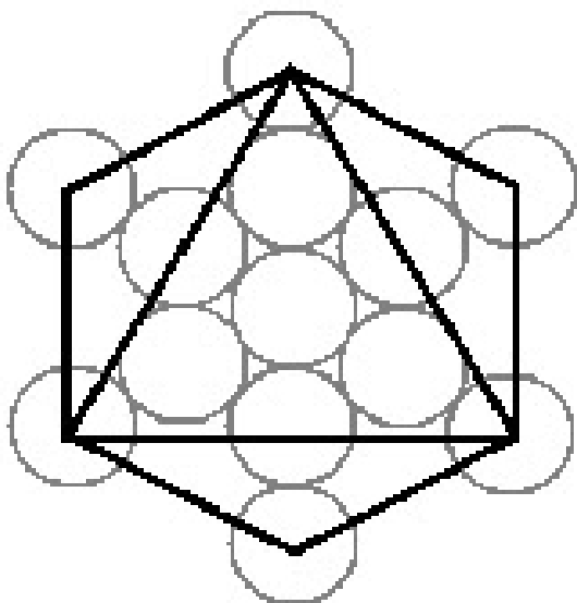
Octahedron
