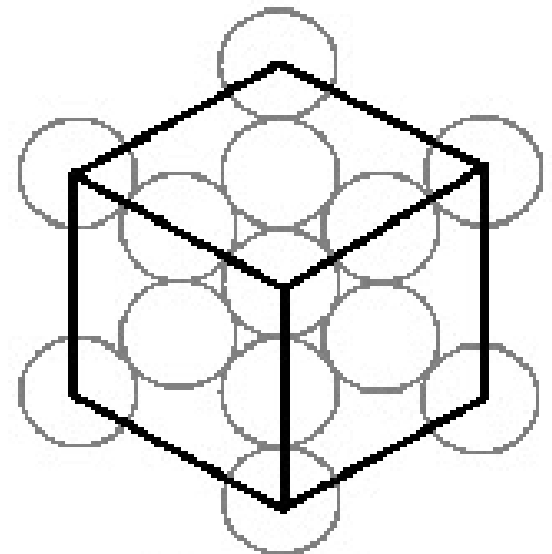
Hexahedron
