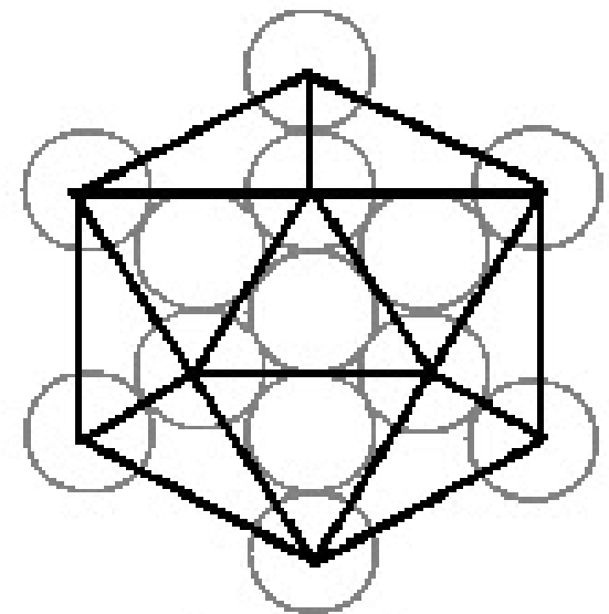
Icosahedron
